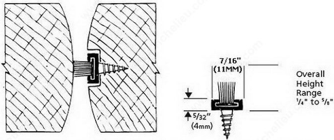
Extruded Aluminum T-Slot Extrusion Drilled & Countersunk w/Fin-Pile Insert
